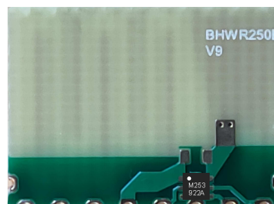
16x12x0.7mm PCBA + BHWM253
